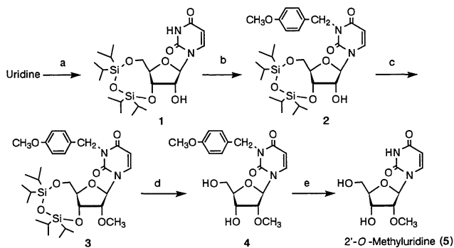
Fig. 2. Reagents and conditions: a. Ref. 1b). b. p -Methoxybenzyl chloride (1.8 equiv), DBU (2.0 equiv), CH 3 CN, 45 °C, 6 h, 92%. c. CH 3 I, Ag 2 O, reflux, 5 h, 100%. d. aq. HF, CH 3 CN, r.t., 94%. e. AlCl 3 (8 equiv), anisole, 65 °C, 2 h, 81%.
